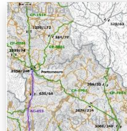
LAYOUT AND DETAIL PROJECT: CONDITIONING OF CP-0701 ROAD. STRETCH: SANTIAGO DE COMPOSTELA - PORTOMOURO
